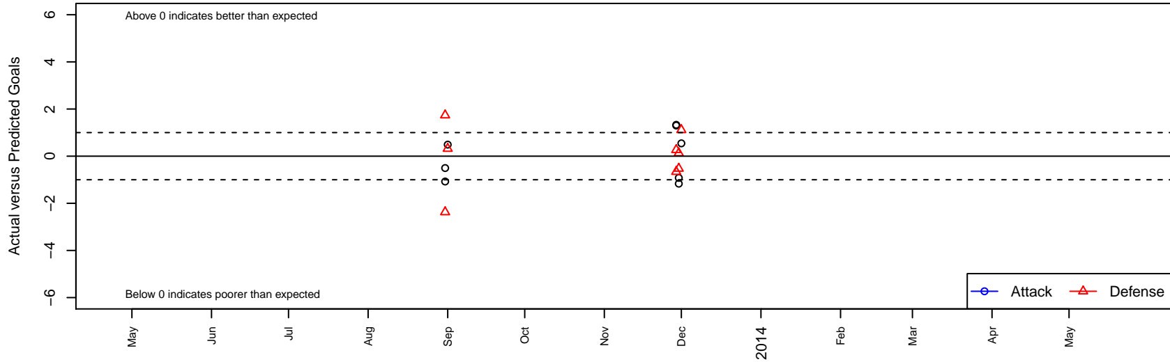
SD Del Sol Lester 03 White G02 Dots are actual minus expected GF (blue circles) and GA (red triangles). Blue line is smoothed change in attack strength. Red is smoothed change in defense strength.
